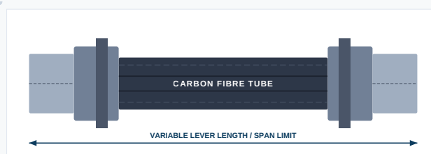
Figure 1: Typical schematic assembly of CENTA Type P carbon fibre high-torque intermediate shaft, exhibiting lightweight mid-section tube integrated with heavy-duty end fittings.
